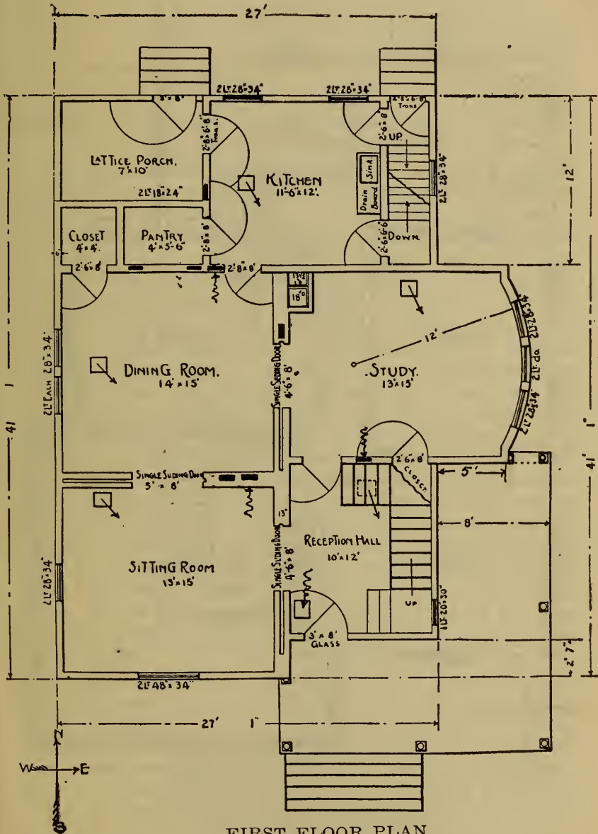
FIRST FLOOR PLAN, Ceiling 10'.
